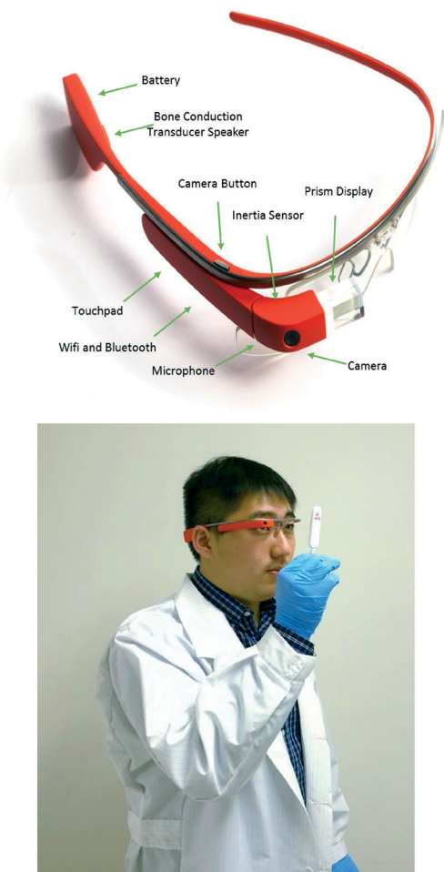
Fig. 4 (Top) Components of Google Glass. 55 (Bottom) Google Glass based imaging and quantification of immuno-chromatographic diagnostic tests. For more details, refer to ref. 56.
